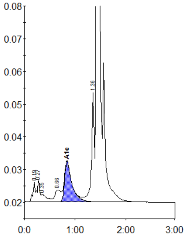
Peak table - ID: 10530185
